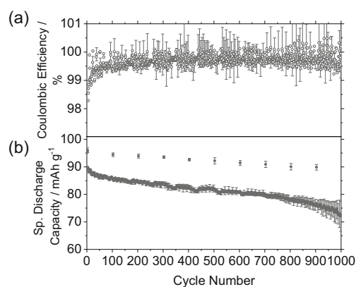
Figure 5. Galvanostatic cycling of graphite || AC half cells ( 5.0\text{--}3.4 \text{ V} vs \text{Li|Li}^+ , three-electrode PAT cell format) using 4.0 \text{ M LiPF}_6 in DMC. WE: graphite, CE: AC, and RE: Li metal. a,b) The C_{\text{eff}} and the specific discharge capacity versus cycle number, respectively. Three formation cycles were performed at 10 \text{ mA g}^{-1} ( \triangleq 0.1\text{C} ). Long-term cycling was performed at 1\text{C} . Every 99 cycles, a characterization cycle was performed at 10 \text{ mA g}^{-1} with a subsequent EIS measurement after charging to 4.6 \text{ V} versus \text{Li|Li}^+ at 10 \text{ mA g}^{-1} . Small capacity and C_{\text{eff}} fluctuations are caused by minor temperature deviations ( (22 \pm 1)^\circ\text{C} ).
