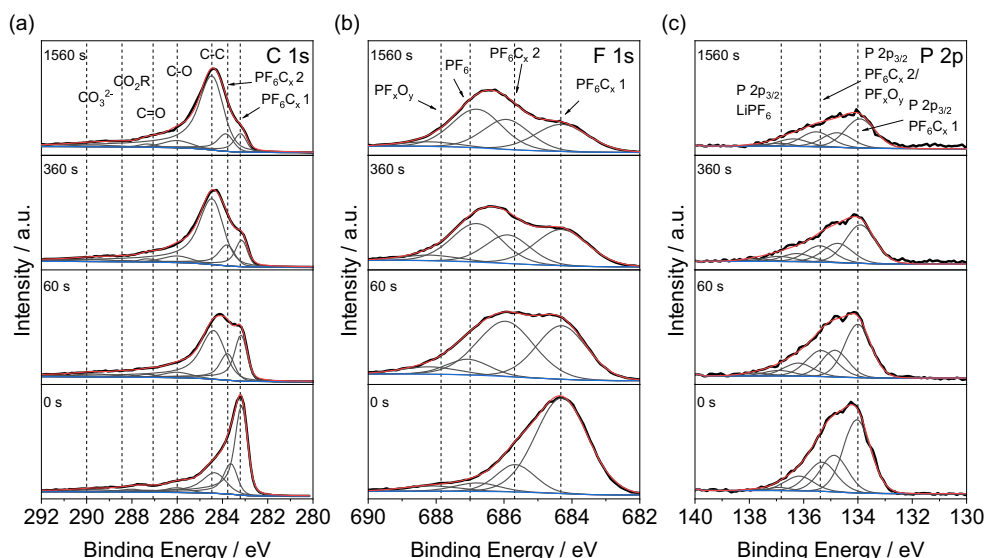
Figure 2. a) C 1s, b) F 1s, and c) P 2p XPS spectra of HOPG charged to 5.0 V versus \text{Li}|\text{Li}^+ at 2 \text{ mA g}^{-1} ( \Delta 0.02\text{C} ) in HOPG || AC cells (Swagelok three-electrode T-cells, half-cell setup). SDP is additionally performed at 0.5 kV with \text{Ar}^+ ions. Total sputter times are indicated as inscriptions in the stacked spectra. Measurements are performed without surface charge compensation. The highly conducting HOPG samples are directly clamped to a bare Cu sample holder to ensure good electronic contact.
